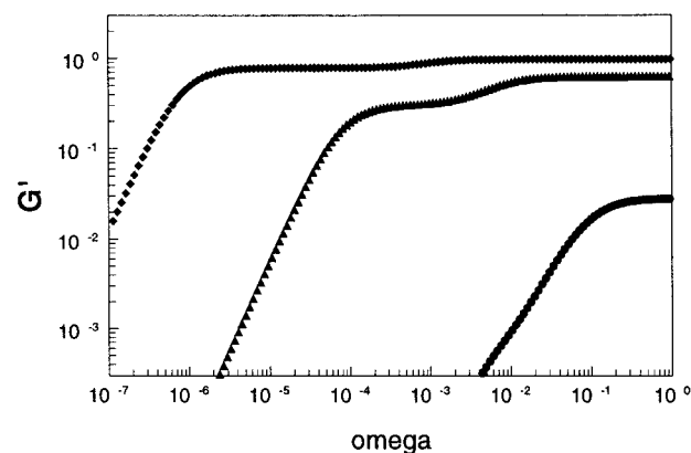
Figure 7. Two types of stickers, N = 6 , E_{g \text{ weak}} = 5 , E_{g \text{ strong}} = 10 : (●) E_{h \text{ weak}} = 3 , E_{h \text{ strong}} = 6 ; (▲) E_{h \text{ weak}} = 5 , E_{h \text{ strong}} = 10 ; (◆) E_{h \text{ weak}} = 7 , E_{h \text{ strong}} = 14 .
